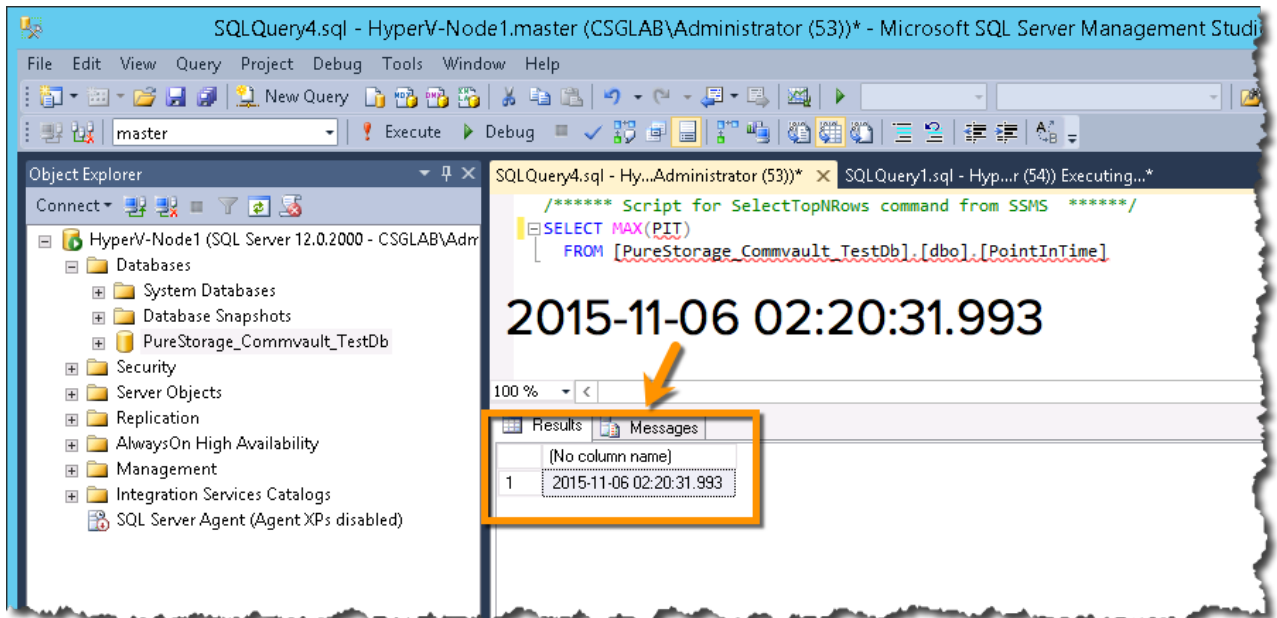
Figure 65. Current Point-in-Time.
