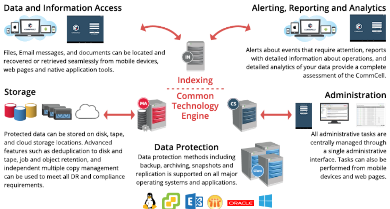
Figure 1. Commvault software.
